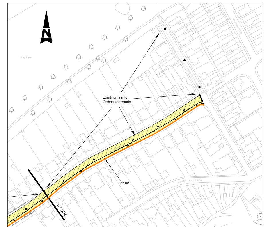
PROPOSED WAITING / LOADING PLAN Scale 1:2000@A1
